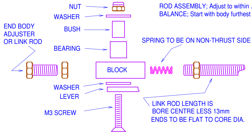
EXPLODED SIDE VIEW OF MICROMETER BLOCK ASSEMBLY
